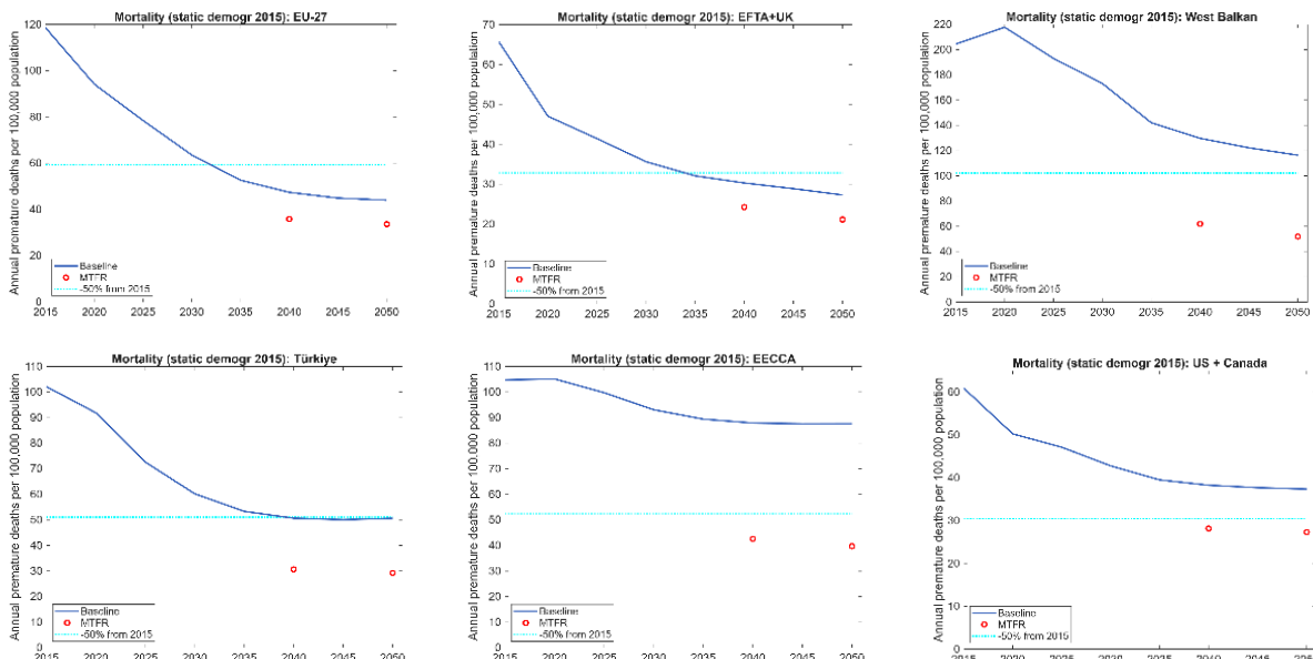
Figure 5: Change in PM 2.5 mortality risks (for the 2015 static population)
