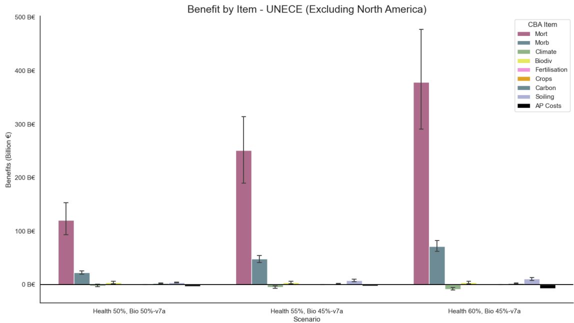
Figure 17: Benefits and additional abatement costs by scenario relative to the baseline scenario in 2040
