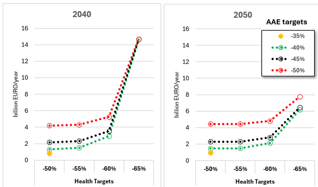
Figure 7: Costs for the range of optimised scenarios in 2040 and 2050 with health ambitions (50-65% risk reduction) on the X-axis. Coloured lines refer to different ambition levels for biodiversity (35-50% risk reduction)
