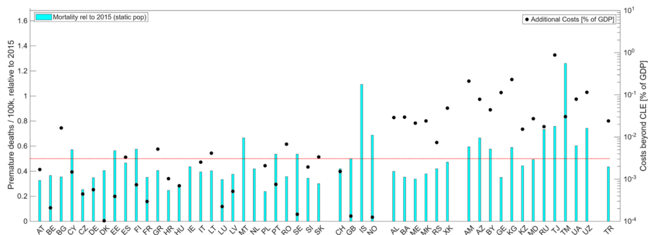
Figure 9: Country outcomes of least cost scenarios for 2040 for a combined 55% risk reduction for health and 45% for biodiversity
