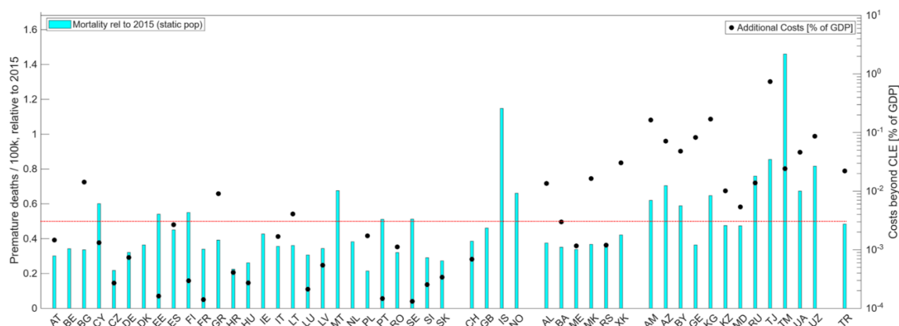
Figure 12: Country outcomes of least cost scenarios for 2050 for a combined 55% risk reduction for health and 45% for biodiversity
