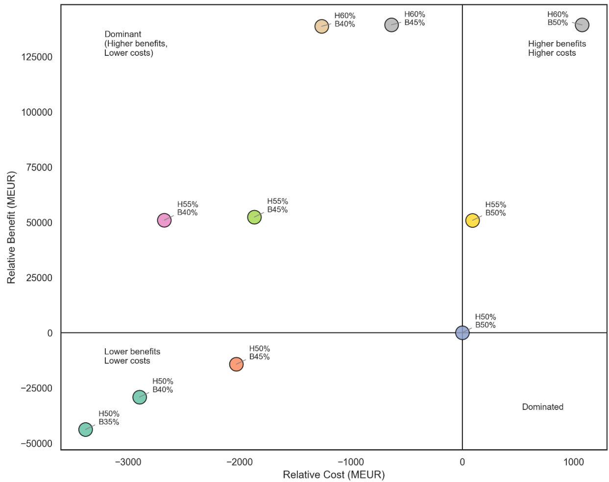
Figure 21: Cost-efficiency plot of the v7a scenarios compared to the 50%/50% scenario
