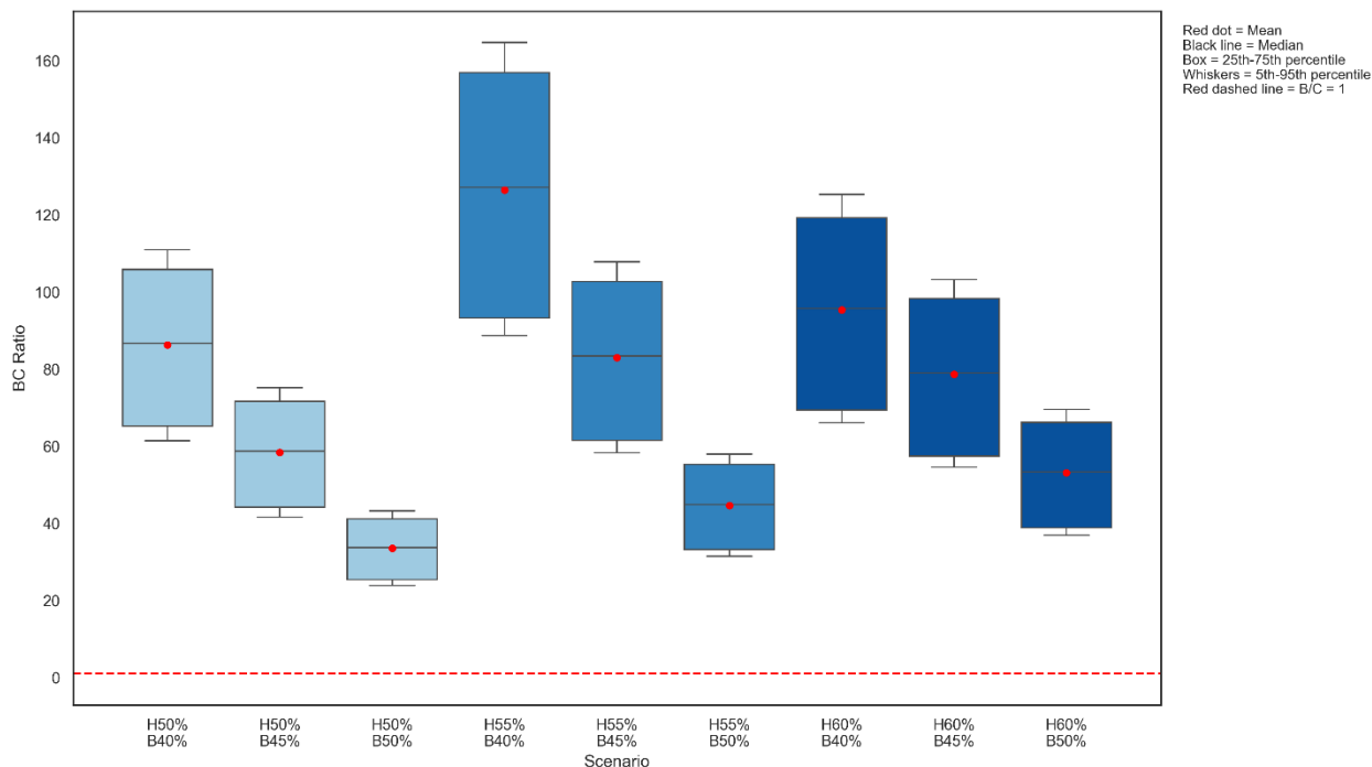
Figure 20: Benefit-cost ratios of the optimised scenarios
