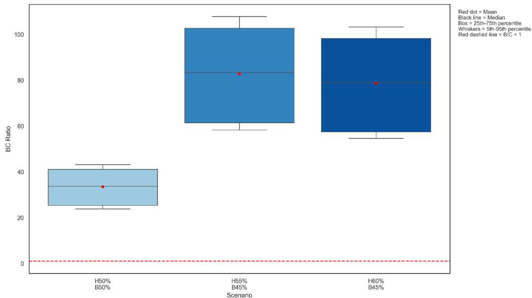
Figure 16: Benefit-cost ratios of the three selected optimized scenarios
