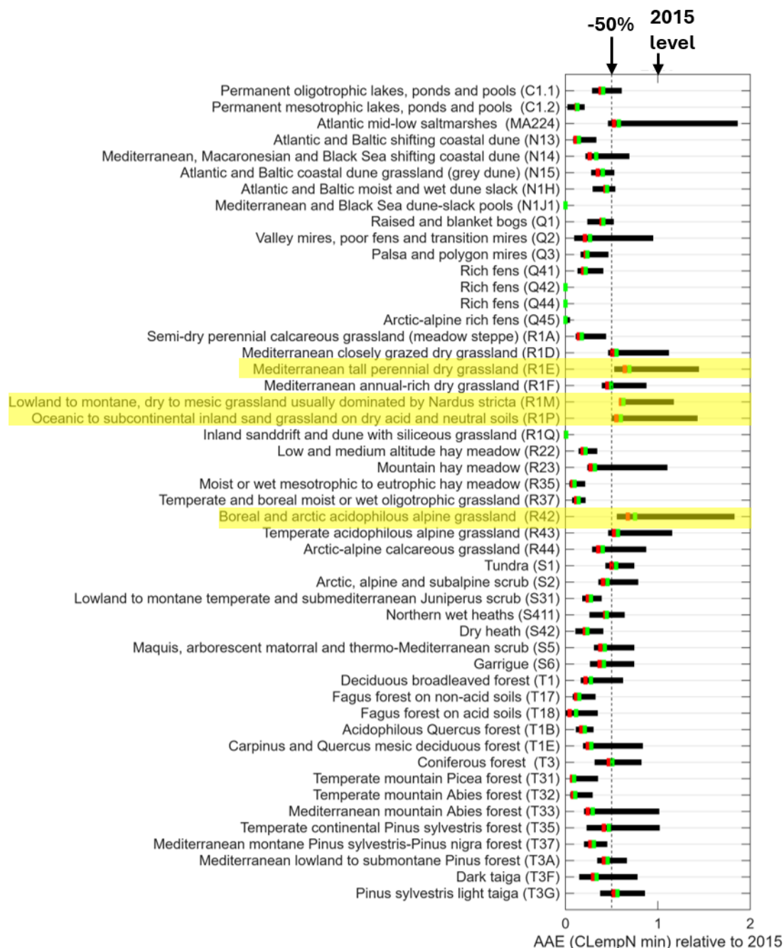
Figure 14: Relative change of biodiversity risk (expressed through AAE) for individual EUNIS habitat types (2040), range between CLE and MTFR (black bars). Results for joint health and biodiversity risk reduction goals: -55%/-45% green, -50%/-50% red. Reduction of risk by 50%, compared to 2015, is not feasible for four ecosystems (marked yellow)
