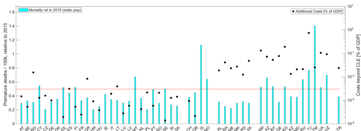
Figure 13: Country outcomes of least cost scenarios for 2050 for a combined 60% risk reduction for health and 45% for biodiversity
