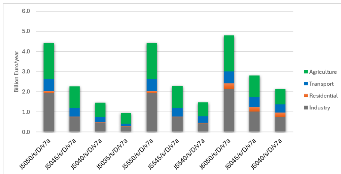
Figure 19: Overview of cost for key sources in optimized scenarios – results for 2050
