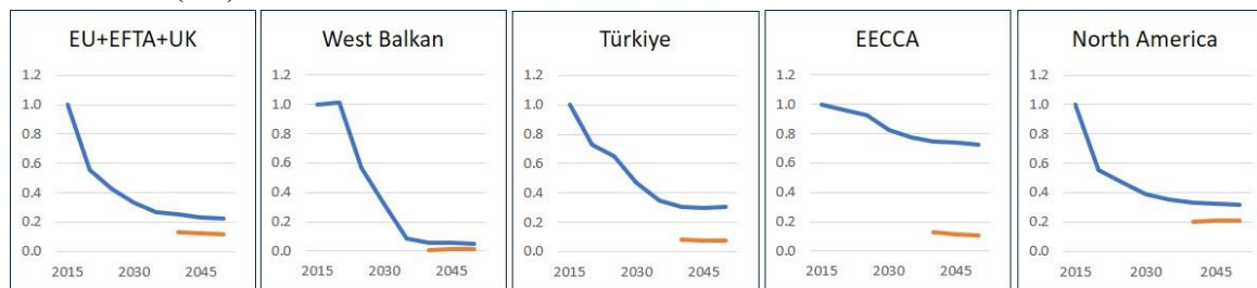
Figure 1: Emission trends, relative to 2015, in Baseline (CLE) and MTR scenario; scenario set v7a
