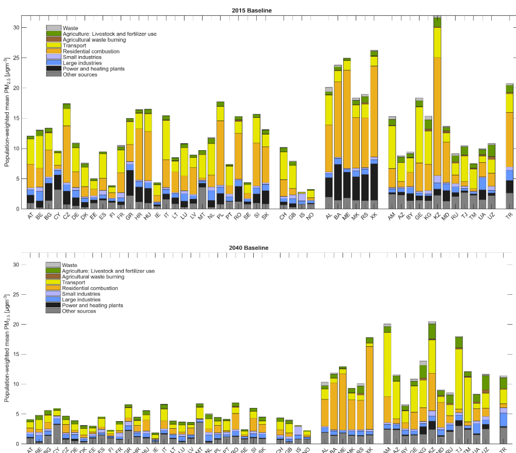
Figure 3: Sector contributions to population weighted country mean anthropogenic PM_{2.5} concentrations in 2015 (top) and according to the baseline in 2040 (bottom), updated to include the sub-grid increment for the full domain
