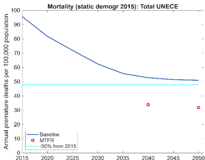
Figure 4: Mortality risk due to anthropogenic PM_{2.5} (annual premature deaths per 100.000 population) in the UNECE-region (incl. North America), using static population. Note: Population data are from UN World Population Prospects 2024 and risk functions from Orellano et al (2024). The illustrative 50% risk reduction target compared to 2015 is shown as the dotted cyan line
