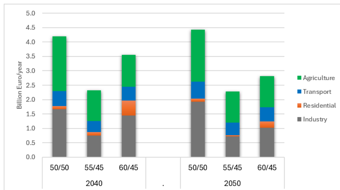
Figure 15: Distribution of costs for key sectors in three selected optimized scenarios
