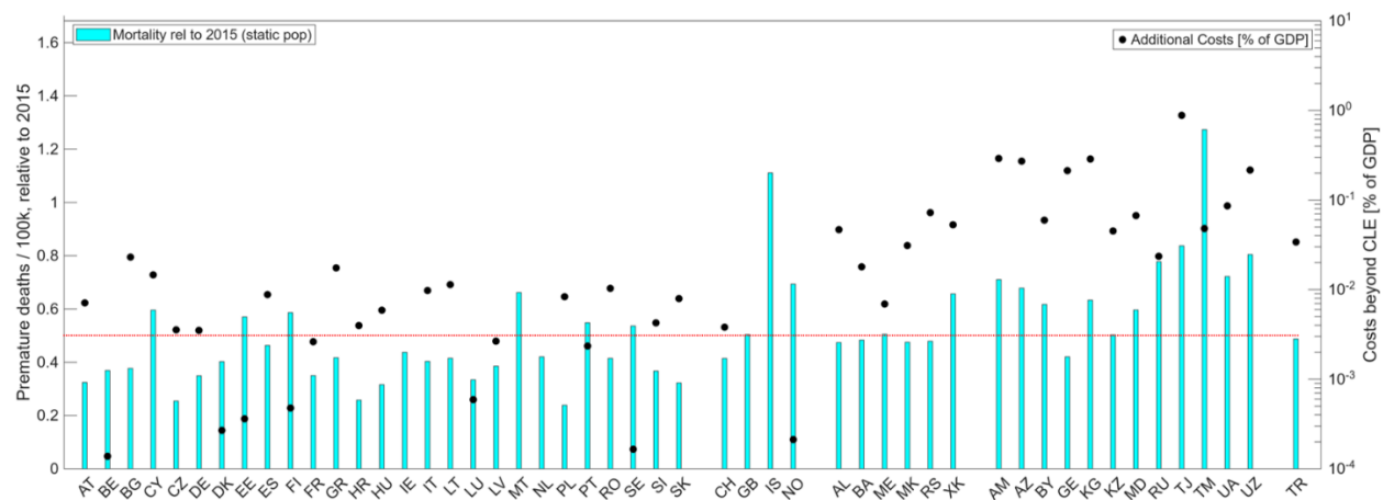
Figure 8: Country outcomes of least cost scenarios for 2040 for a combined 50% risk reduction for health and biodiversity
