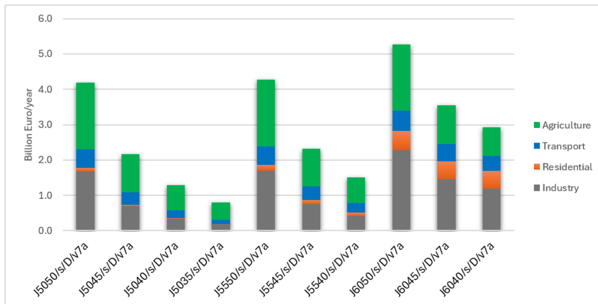
Figure 18: Overview of cost for key sources in optimized scenarios – results for 2040
