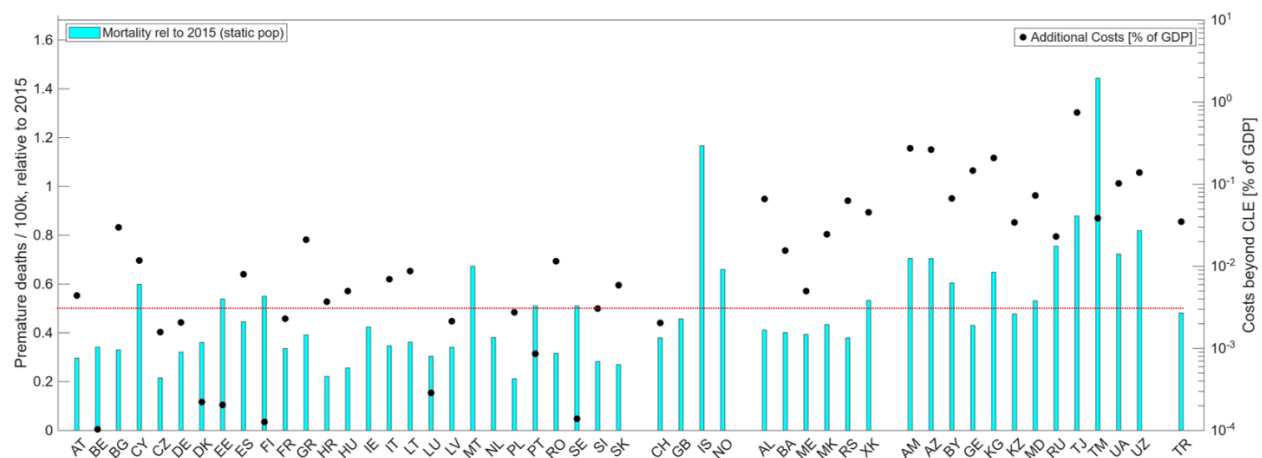
Figure 11: Country outcomes of least cost scenarios for 2050 for a combined 50% risk reduction for health and biodiversity
