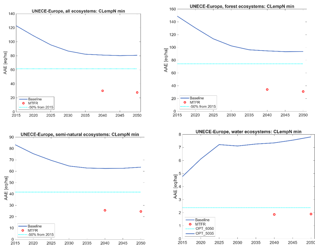
Figure 6: Attainability of 50% reduction of the average accumulated exceedance of the minimum nitrogen critical loads (CLempN min) for specific ecosystems in the UNECE (excl. NA, but including non-Parties to the Air Convention 7 )
