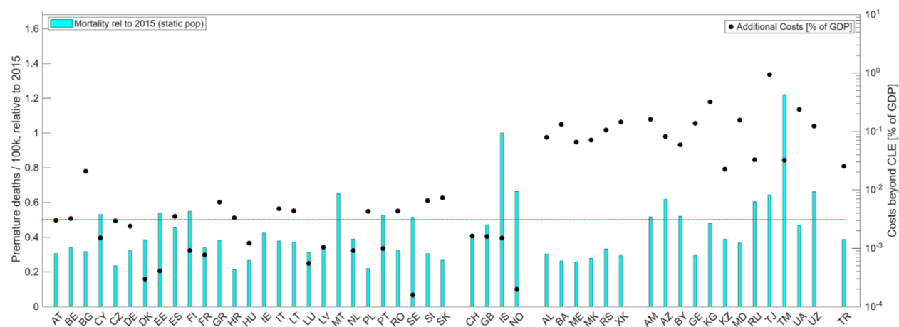
Figure 10: Country outcomes of least cost scenarios for 2040 for a combined 60% risk reduction for health and 45% for biodiversity
