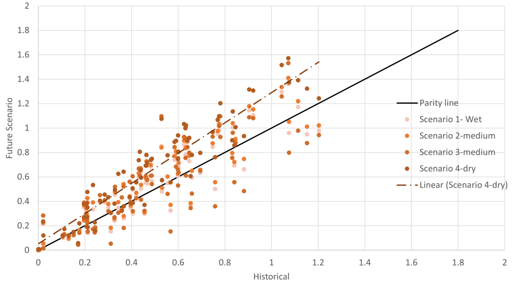
Mean difference between annual maximum and annual minimum Watertable (meters)
